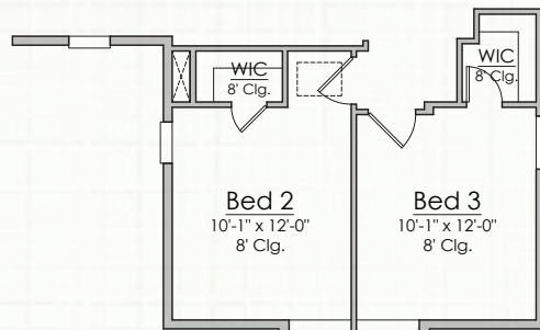
Elevation B 2nd Floor Plan (+6 Sq.Ft.)
