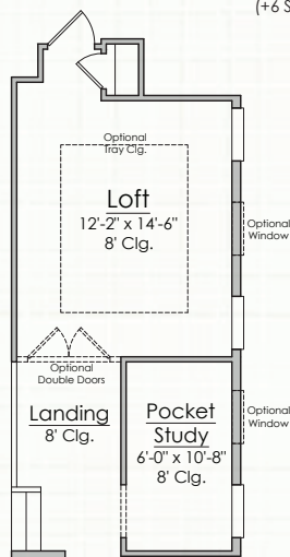
Optional Full Wall at Loft
