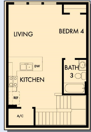
OPTIONAL SECOND FLOOR WITH LIVING, KITCHEN, BEDROOM 4 AND BATH 3 ABOVE GARAGE
