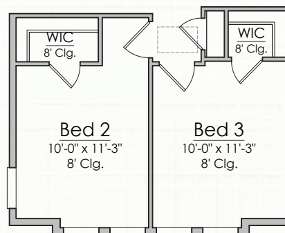
Elevation C 2nd Floor Plan (+4 Htd.Sq.Ft.)
