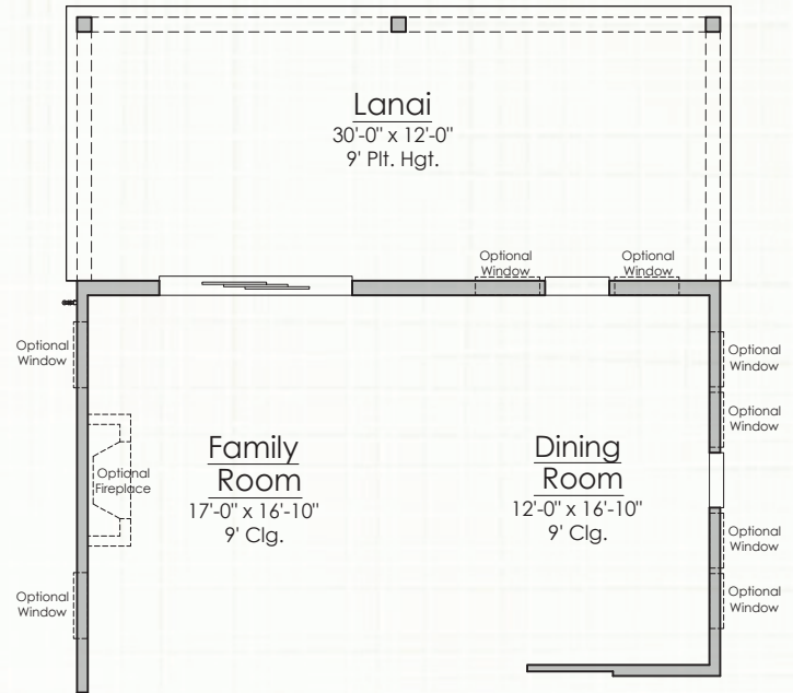
Optional Super Lanai +261 Sq.Ft. at Lanai
