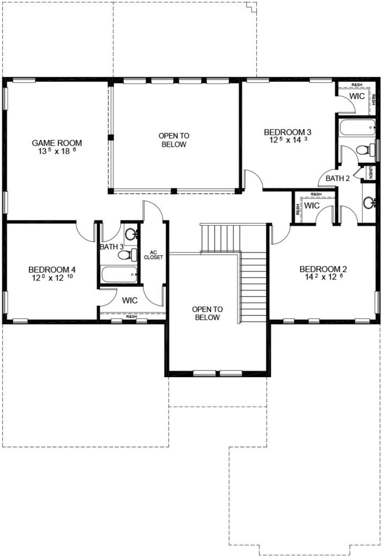
SECOND FLOOR
